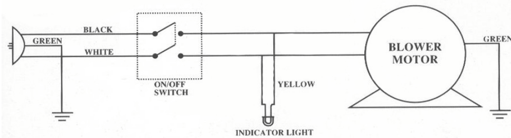
Single Phase Schematic
