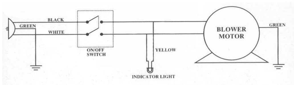
Single Phase Schematic
