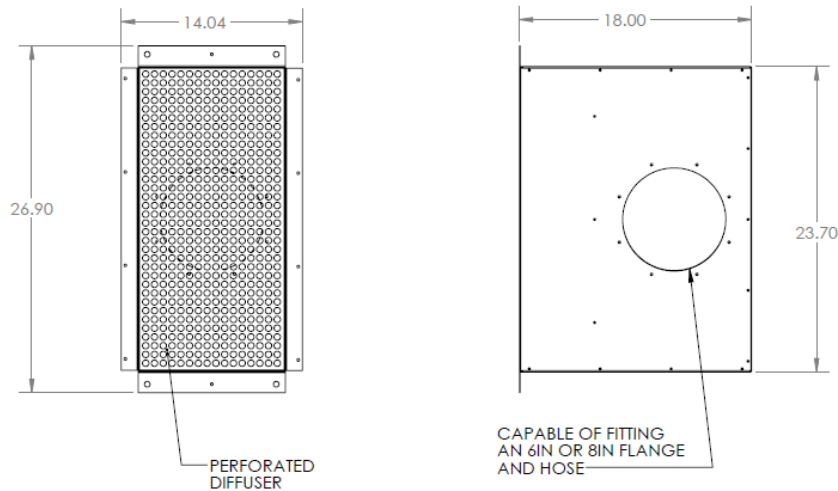
FIGURE 11- F33 SOURCE CAPTURE PLENUM DIMENSIONS
