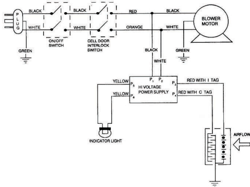
SINGLE PHASE
