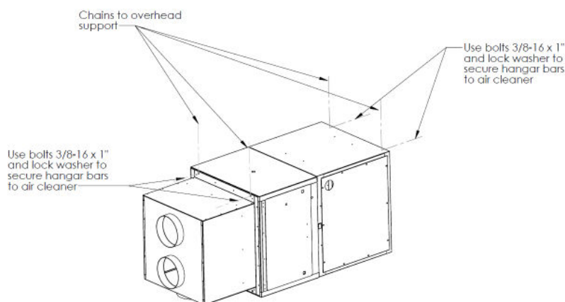
FIGURE 10 – MOUNTING F66 OVERHEAD F73 USES 3/8" EYEBOLTS PROVIDED
