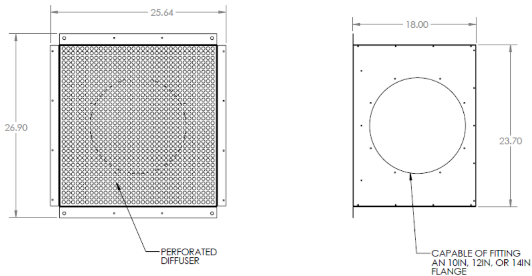
FIGURE 11 – F66 SIZE SOURCE CAPTURE PLENUM DIMENSION
