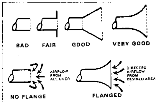
FIGURE 7 – HOOD FLANGES
