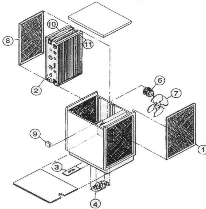
FIGURE 8 – RespirAide PARTS LIST
