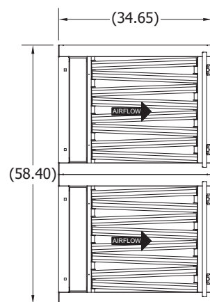
AUTOCLEAN® 8000 & F72C Odor Control Module Side View (Facing Access Door)
