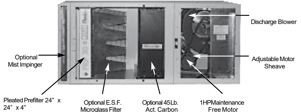
M66L SHOWN WITH OPTIONAL 45 LB. CARBON MODULE & E.S.F. FILTER
