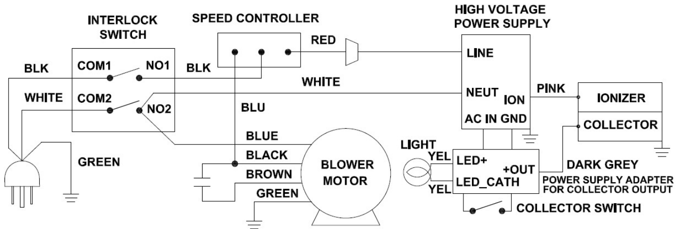
MB500 Schematic
