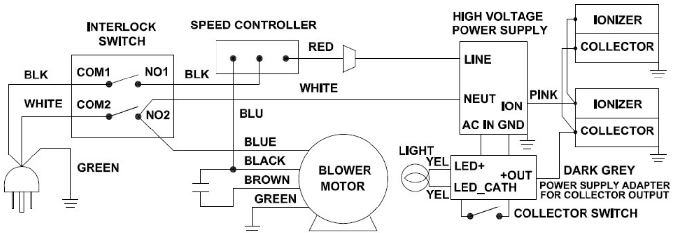
MB850C Schematic
